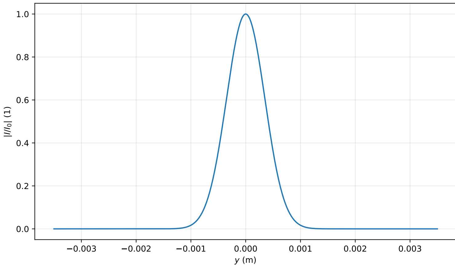
Intensity profile I(x = 0, y, z = 0.000)/I_0 , P_{in}=0.3P_{cr} , artificial time
